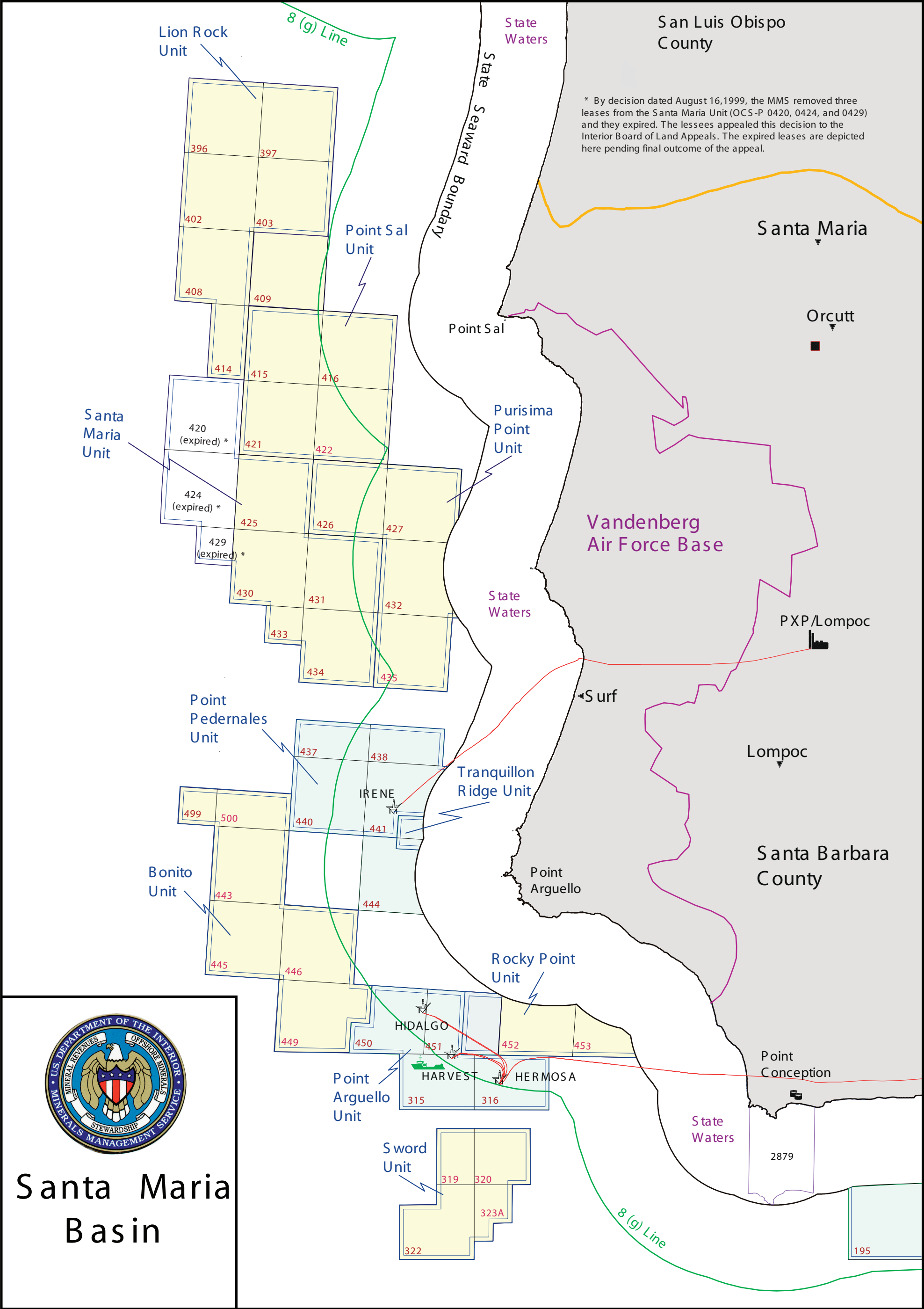
Figure 1. Location of Units and Lease OCS-P 0409 in the Santa Maria Basin.
